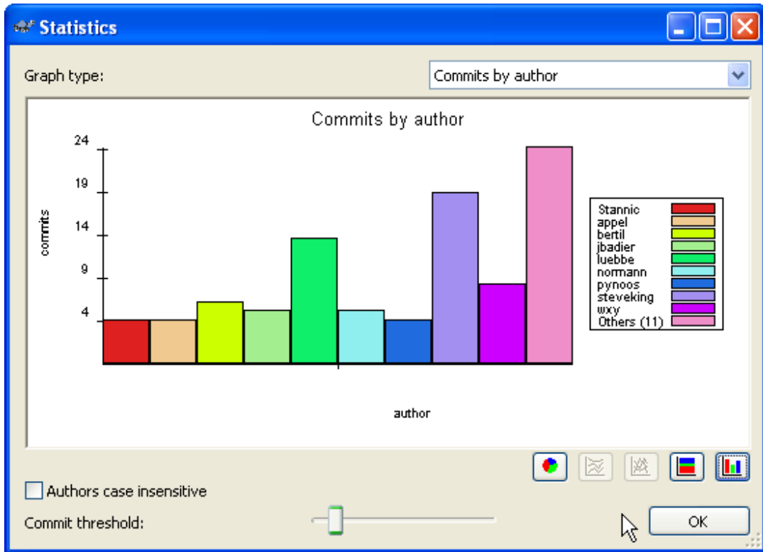
Figure 5.18. Commits-by-Author Histogram
