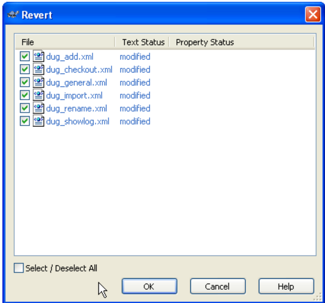
Figure 5.26. Revert dialog
