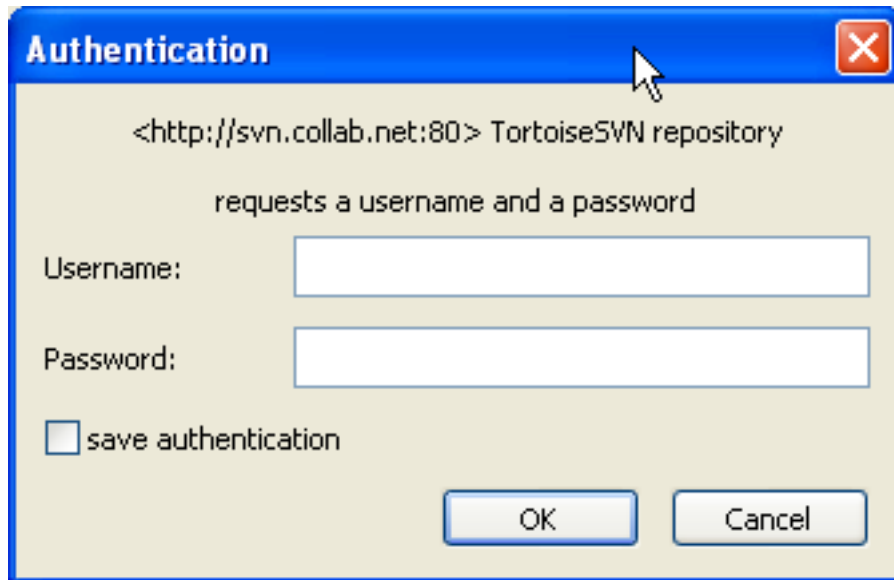
Figure 5.5. Authentication Dialog
